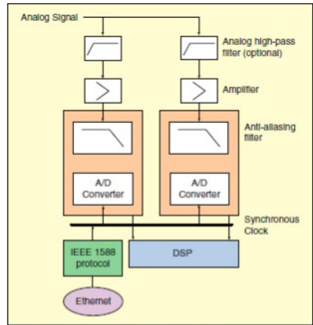
Figure 10. Input front-ends in one hardware module.
