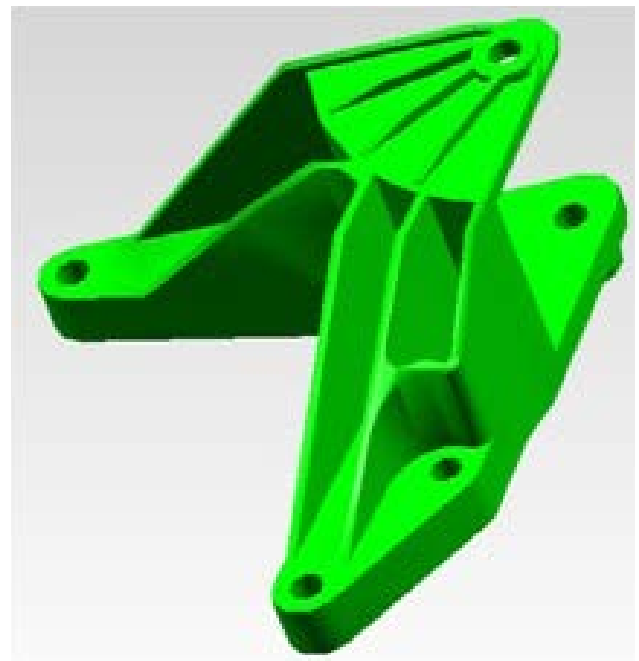
Figure 1.6 Pro/E 3D model
