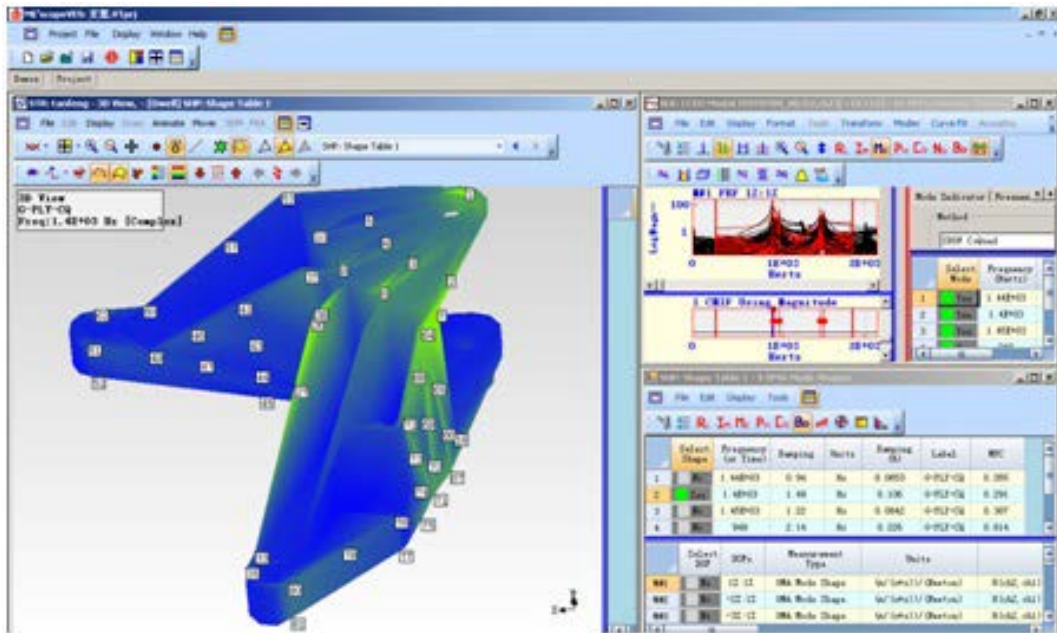
Figure 1.8 Modal data display window in ME'Scope
