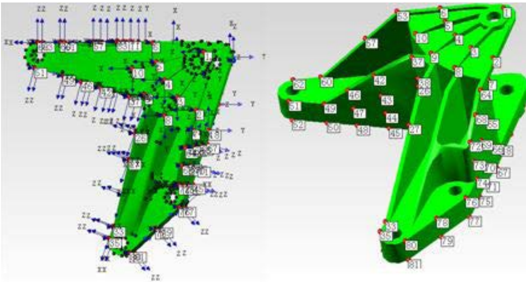
Figure 1.7 Excitation point locations and directions
