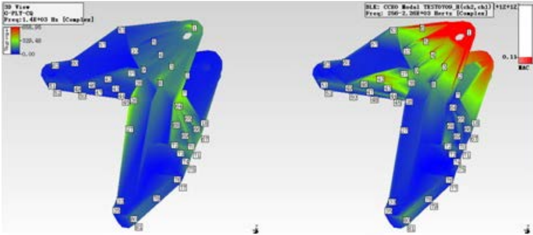
Figure 1.9 ME'Scope display of modes
